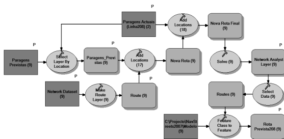
Figure 5 - Example in model builder of a previews work of the recalculation of the bus routes
